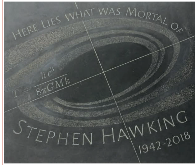
Tombstone of Stephen Hawking's grave in Westminster's Abbey, containing his ashes. At his 60th birthday in 2002, Hawking requested equation (10.165) to be engraved on his tombstone.
