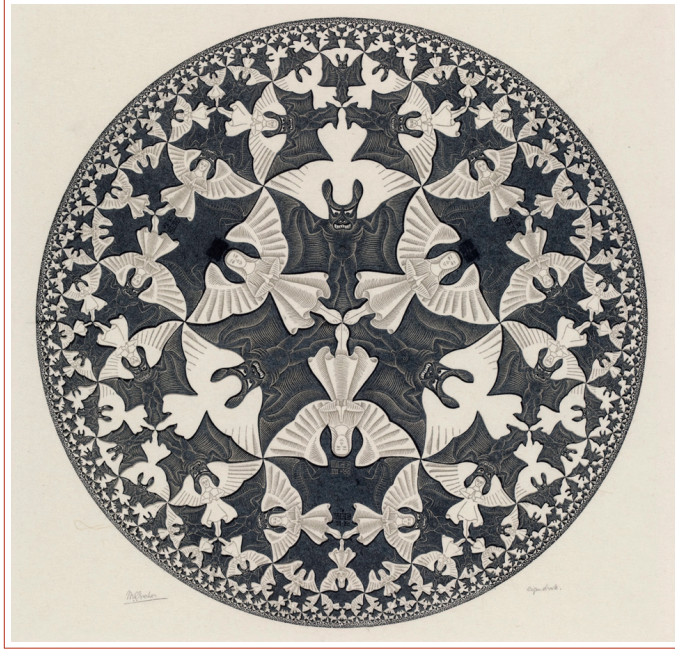
Circle Limit IV (Heaven and Hell) by M.C. Escher, showing the Poincaré disc
