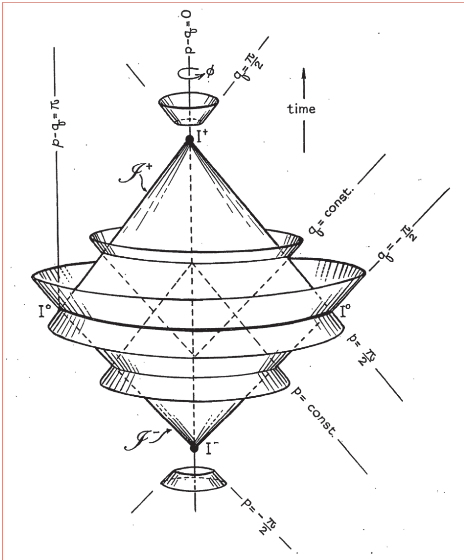
The conformal completion (\hat{\mathbb{M}}, \hat{\eta}) of Minkowski space-time (\mathbb{M}, \eta) , with the \theta -coordinate suppressed, taken from Penrose (1964). Future timelike infinity I^+ , past timelike infinity I^- , and spacelike infinity I^0 (called i^+ , i^- , and i^0 in the main text, following current notation), are drawn, but do not belong to \hat{\mathbb{M}} . Likewise, the shells at p > \frac{1}{2}\pi and q < -\frac{1}{2}\pi are not part of \hat{\mathbb{M}} , which “ends” at I^0 and is a rotated diamond without the equatorial circle and north and south poles; they are just drawn to clarify the meaning of the coordinates. Also, the caps above I^+ and below I^- are not part of \hat{\mathbb{M}} . Metrically I^0 is a point, like I^+ and I^- , rather than a circle.
